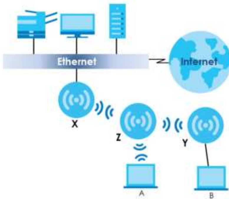
Figure 5 Repeater Application
