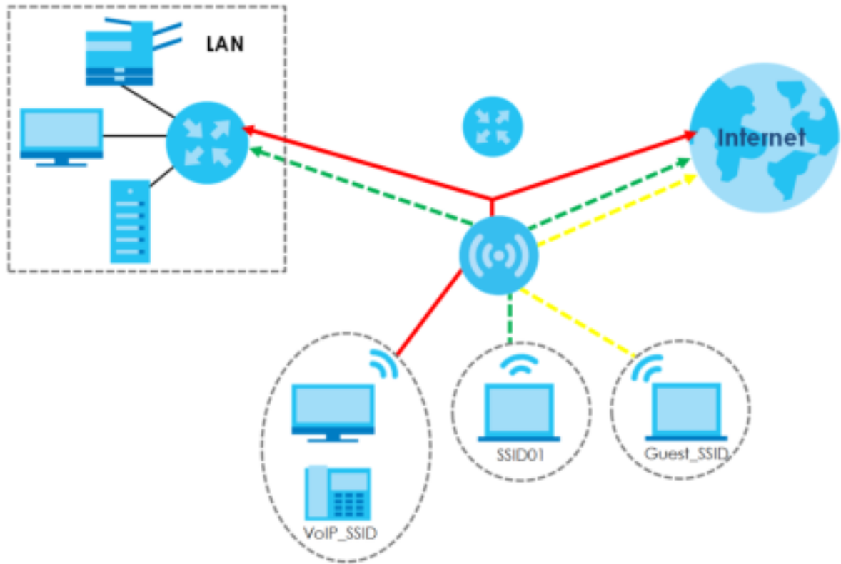
Figure 6 Multiple BSSs
