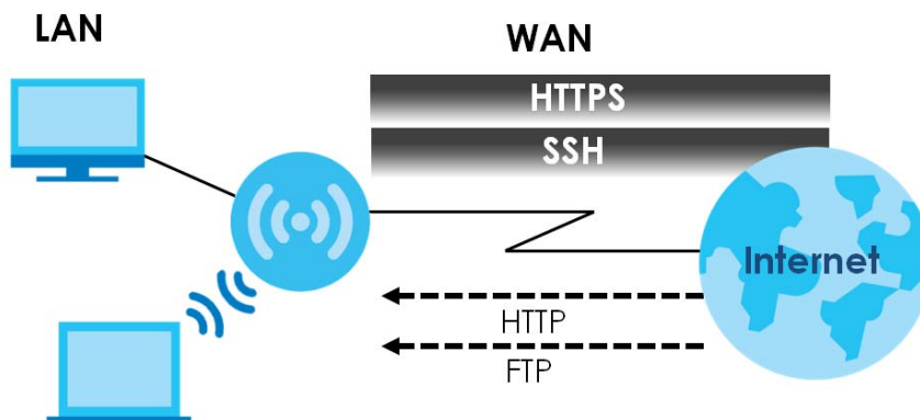
Figure 114 Secure and Insecure Service Access From the WAN
