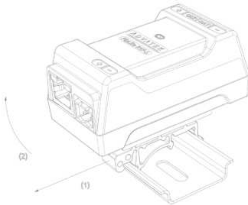
Figure 5: Removal of Receiver from DIN Rail
