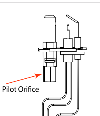
Figure 26: Pilot Assembly
