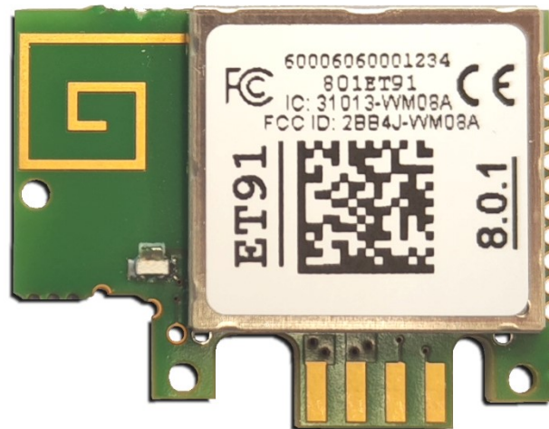
Picture Modul 868MHz VIII top-side
