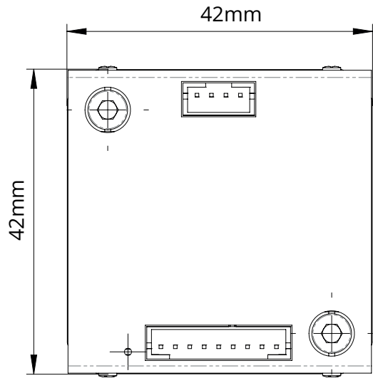
Figure 5: TCM-1070 top view mechanical dimensions
