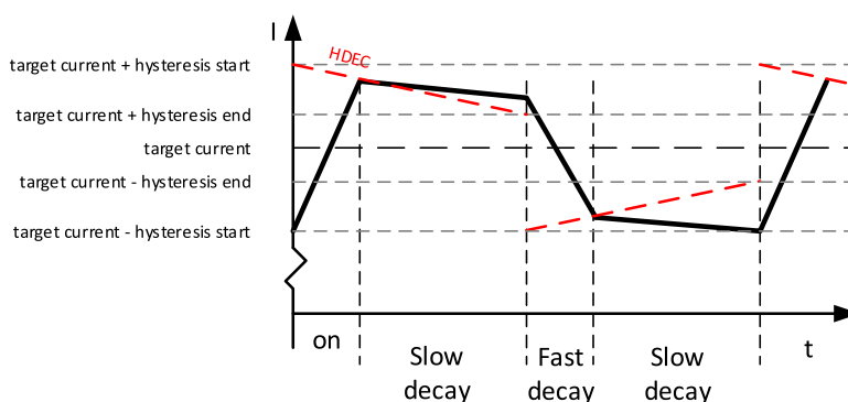
Figure 2: spreadCycle principle
