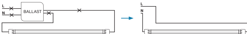
Wiring Diagram B: Shunted Double-Ended Wiring
