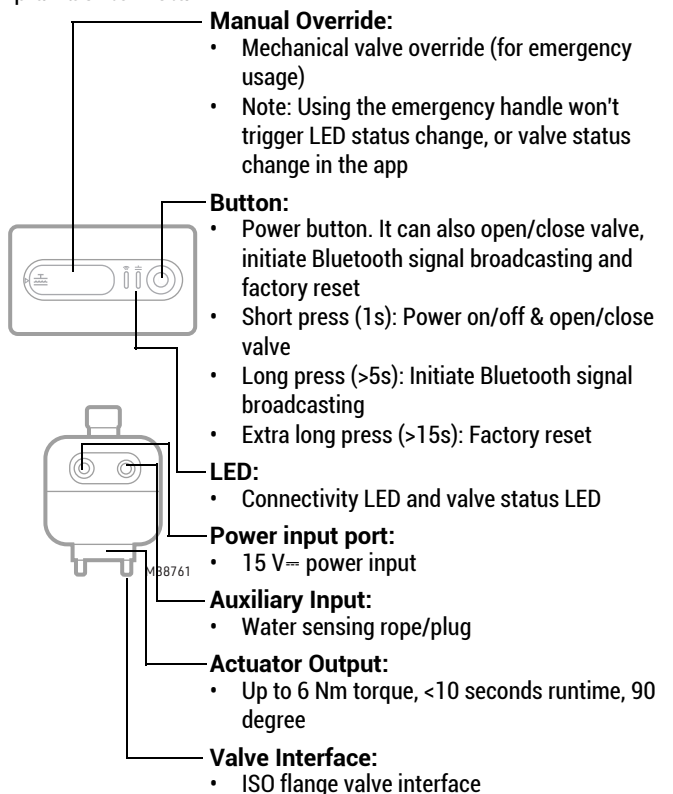
Fig. 2. Components.
