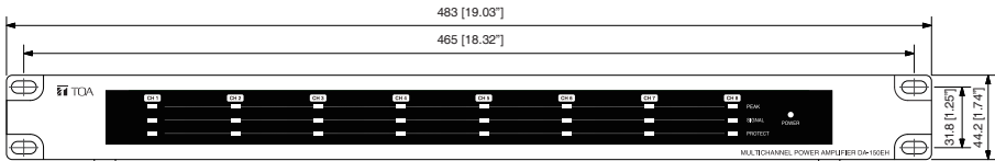
Front View
