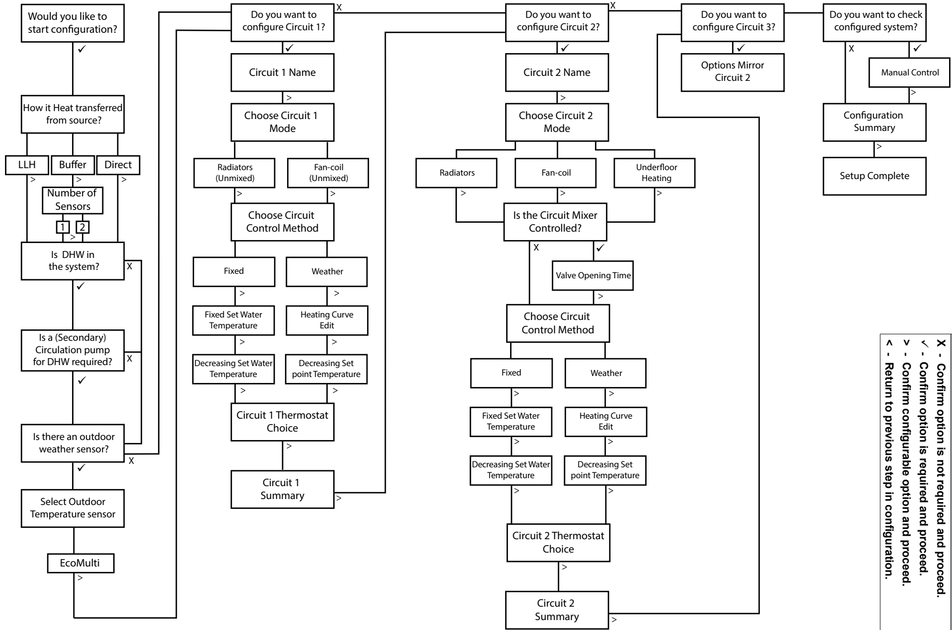
Figure 6-6: System Configuration Map
