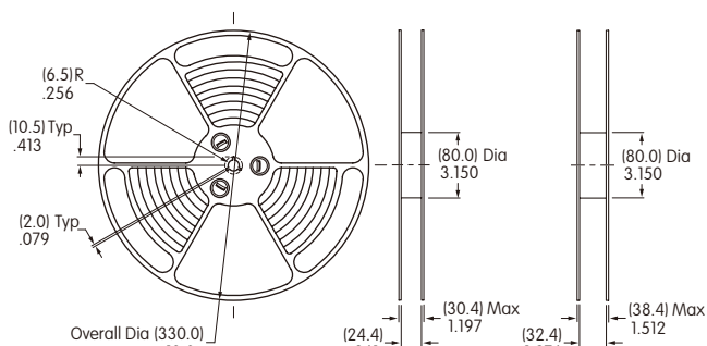
Reel Dimensions JS0204AP4-R JS0208AP4-R
