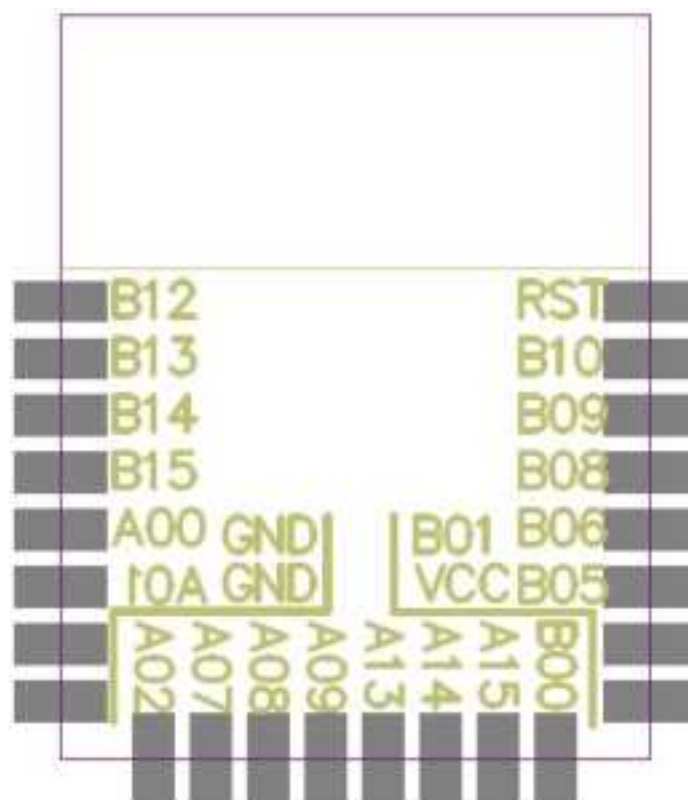
Figure 2 Top View
