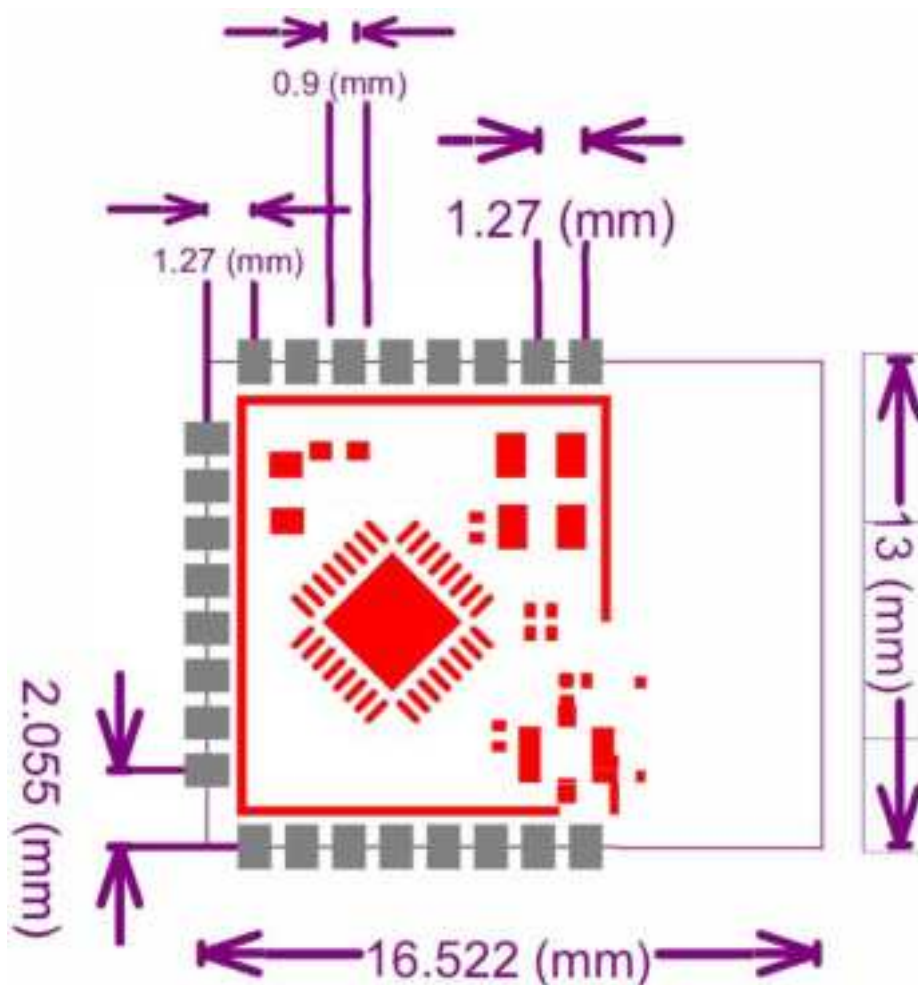
Figure 1 Chip Dimensions
