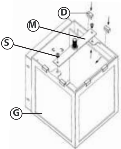
Drawing 3-Glass install
