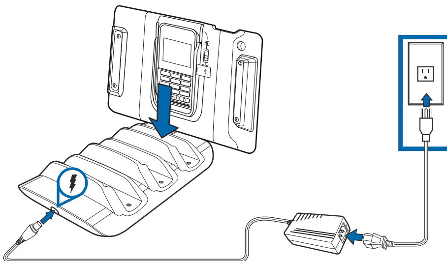
Figure 29 Using the Gang Charger
