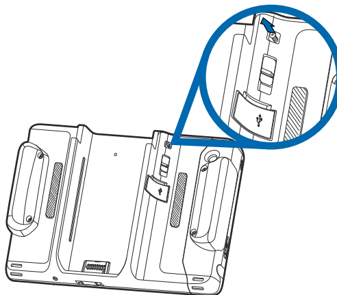
Figure 13 Loosening Screw to Unlock Release Button
