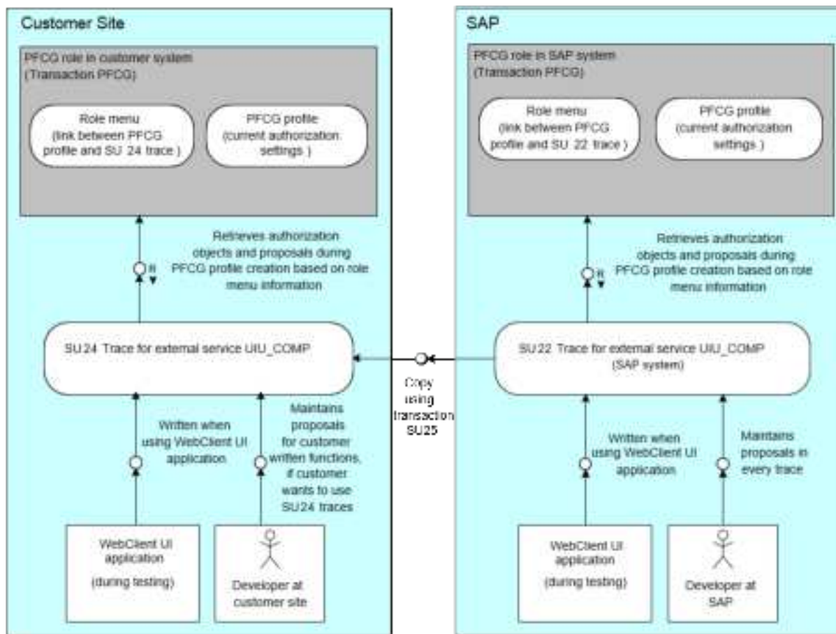
Dependencies
