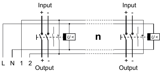
Wiring diagram of fireman's switch SOL30X...-SAFETY
