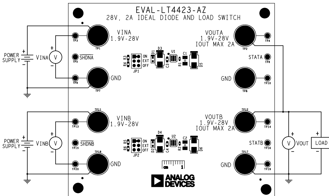
Figure 1. EVAL-LT4423-AZ Board Connection in Diode-Or Configuration
