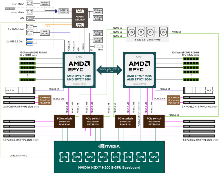
G893-ZD1-AAX5 System Block Diagram
