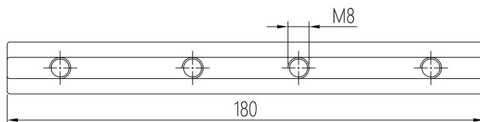
Straight Connector
