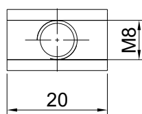
Spring Nut: M8
