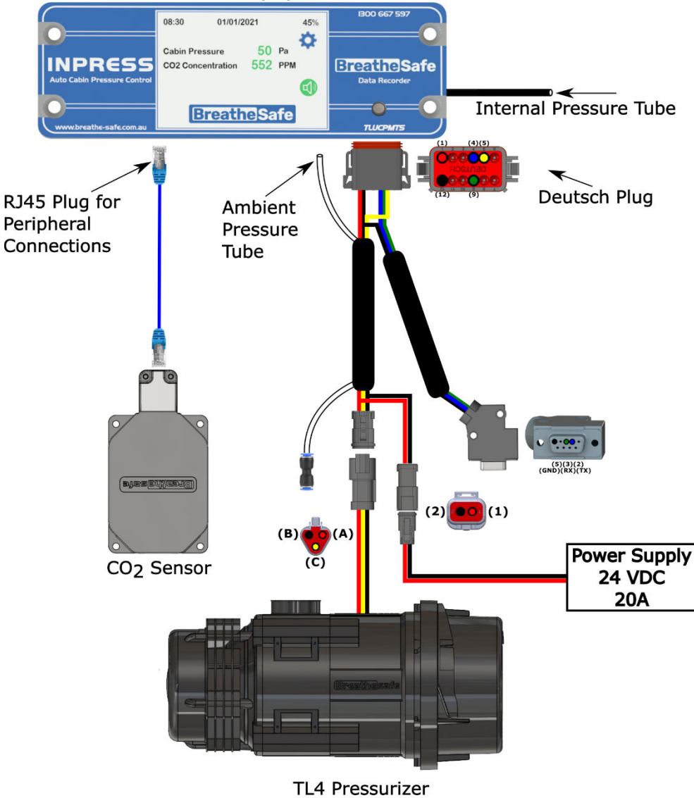
INPRESS User Interface (UI)
