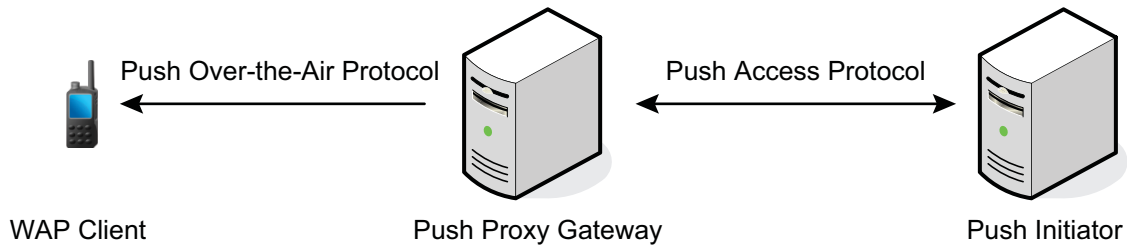
Figure 19: Push Framework
