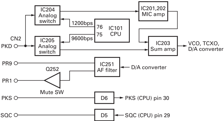
Fog. 17 Data terminal and peripheral circuits
