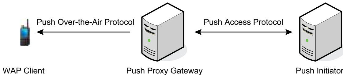
Figure 14: Push Framework
