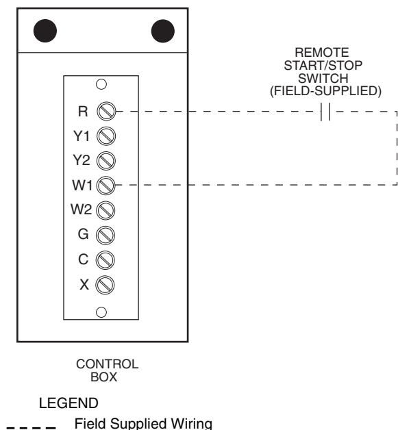
Fig. 26 — Field Control Remote Start/Stop
