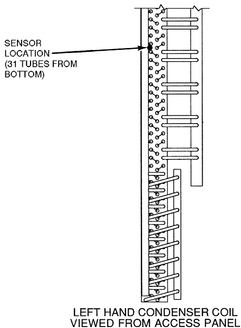
Fig. 53C — Motormaster III Sensor Location (48AJ,AK,AW,AY040, 050 and 48EJ,EK,EW,EY048)
