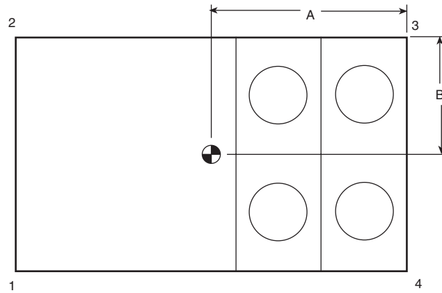
48AJ,AK,AW,AY UNITS
