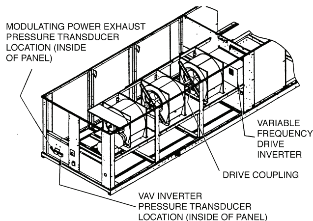
Fig. 51 — Pressure Transducer Locations (48AJ,AK,AW,AY060 and 48EJ,EK,EW,EY054-068)
