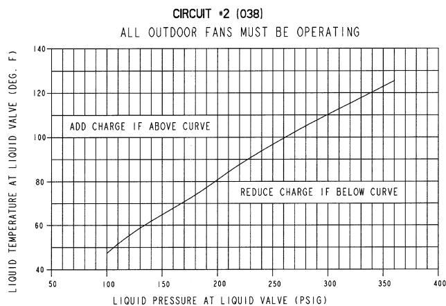
Fig. 72 — Cooling Charging Chart, 48EJ,EK,EW,EY038-048
