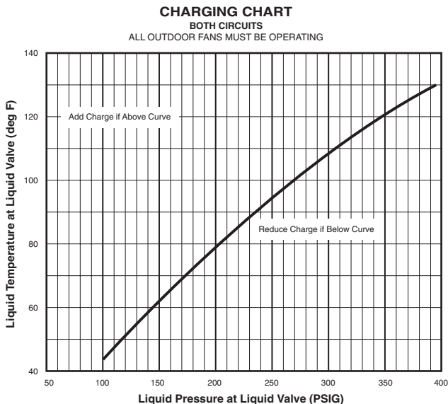
Fig. 74 — Cooling Charging Chart, 48AJ,AK,AW,AY020-060
