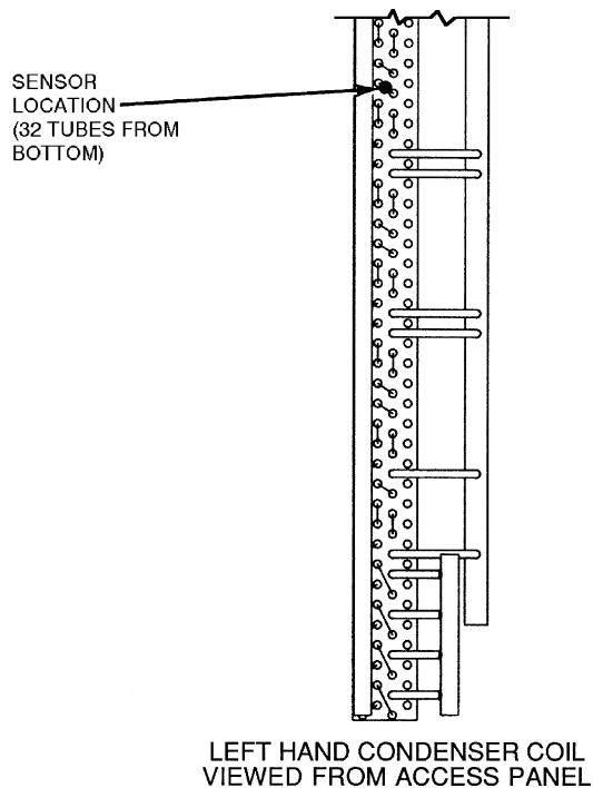
Fig. 53B — Motormaster® III Sensor Location (48AJ,AK,AW,AY035 and 48EJ,EK,EW,EY038, 044)
