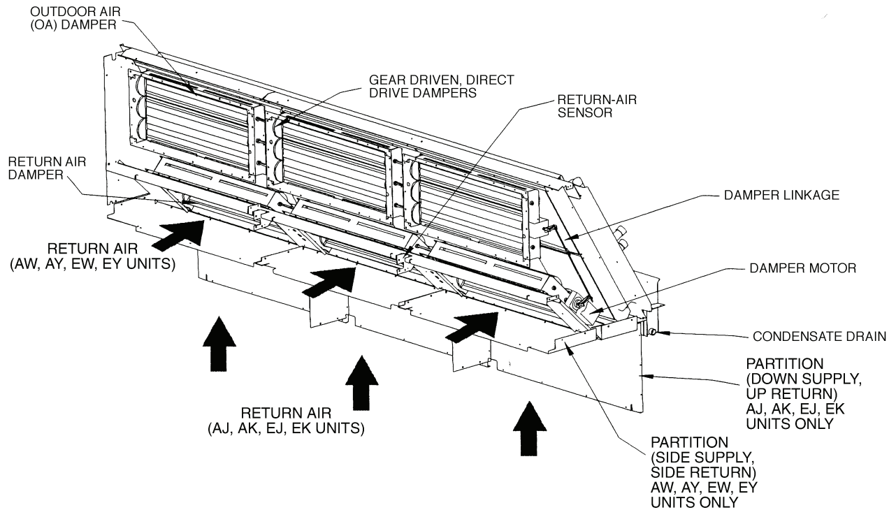
Fig. 49 — Economizer Details
