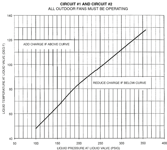
Fig. 73 — Cooling Charging Chart, 48EJ,EK,EW,EY054-068
