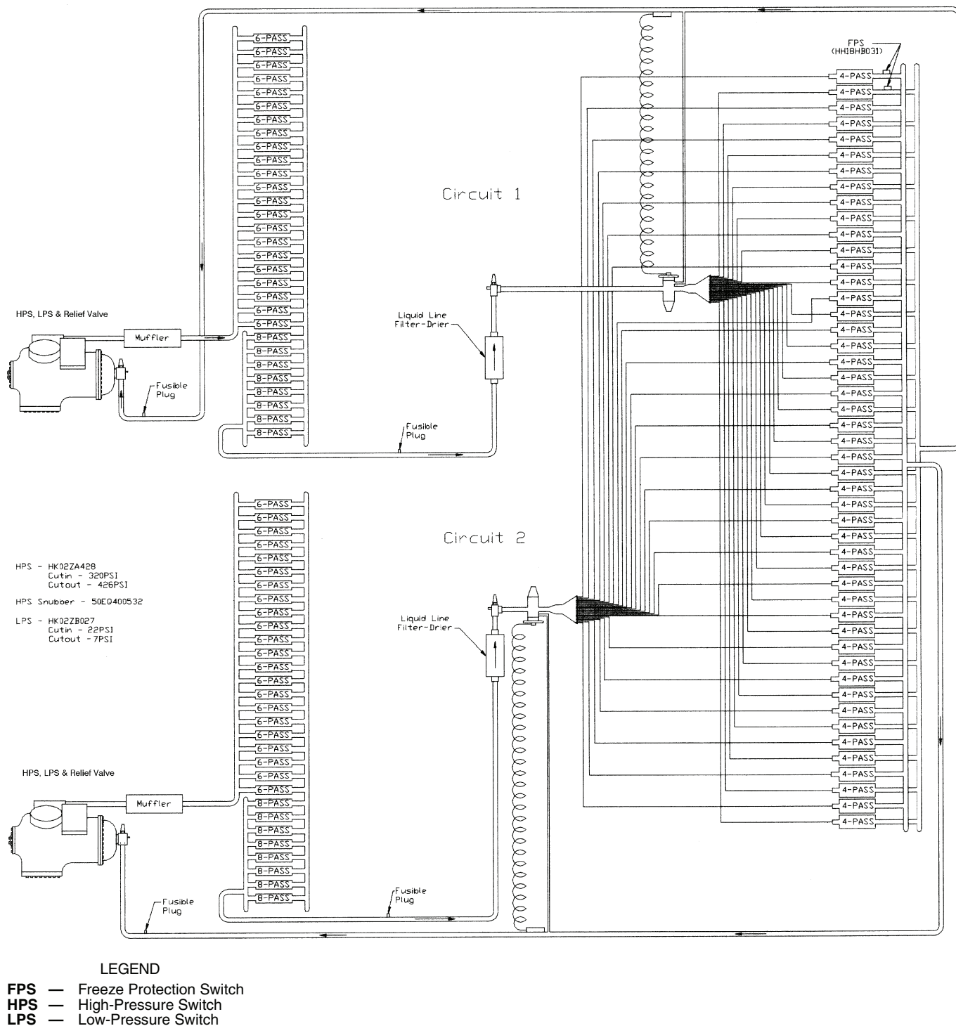
Fig. 89 — Typical Refrigerant Circuiting (48EJ,EK,EW,EY048)
