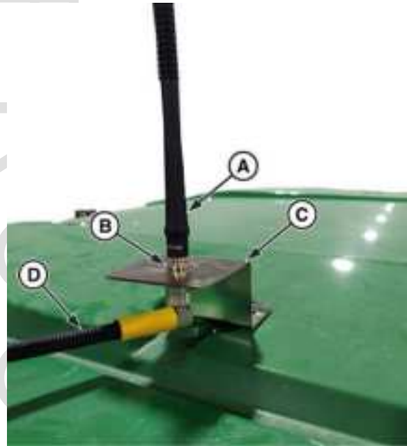
Antenna Installation
