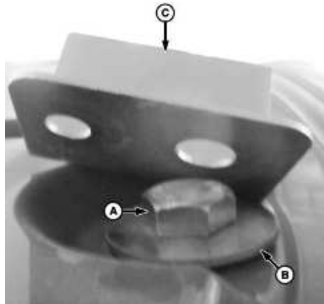
Antenna Bracket Installation
