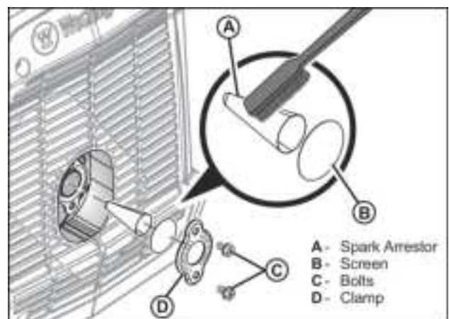
Figure 44 Remove and Clean the Spark Arrestor
