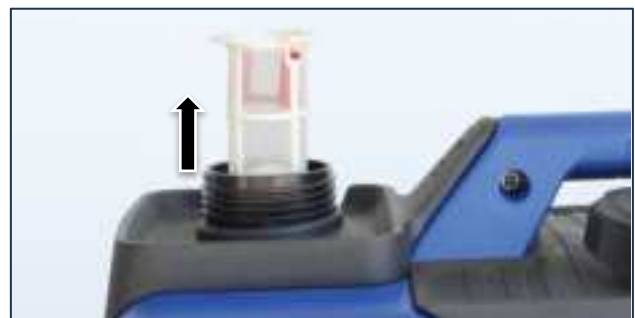
Figure 33 Remove the Fuel Strainer
