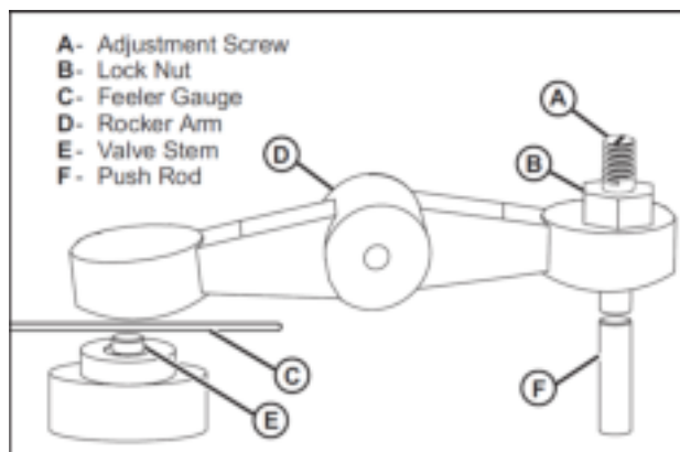
Figure 46 Set Valve Clearance
