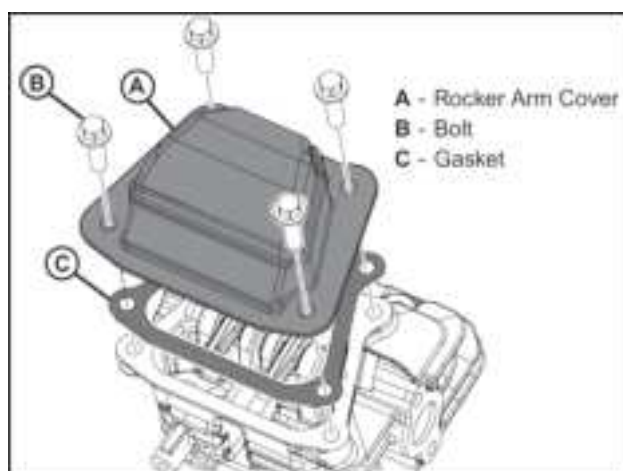
Figure 45 Remove Rocker Arm Cover
