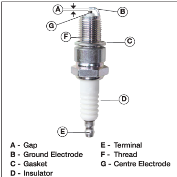
Figure 42 Spark Plug
