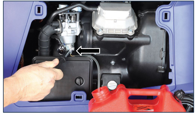
Figure 36 Drain the Carburettor
