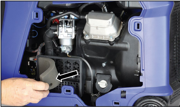
Figure 32 Remove the Air Filter Element
