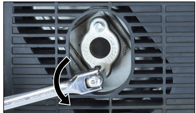
Figure 43 Remove the Spark Arrestor Clamp
