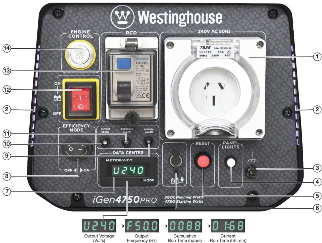
Figure 4 iGen4750PRO Control Panel Features
