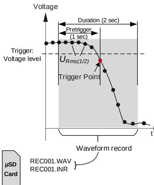
Figure 5.19: Voltage Level Triggering
