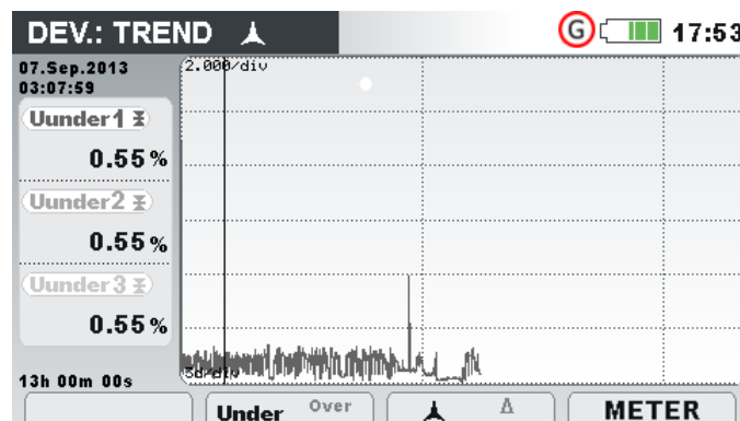
Figure 3.42: Underdeviation and overdeviation TREND screen
