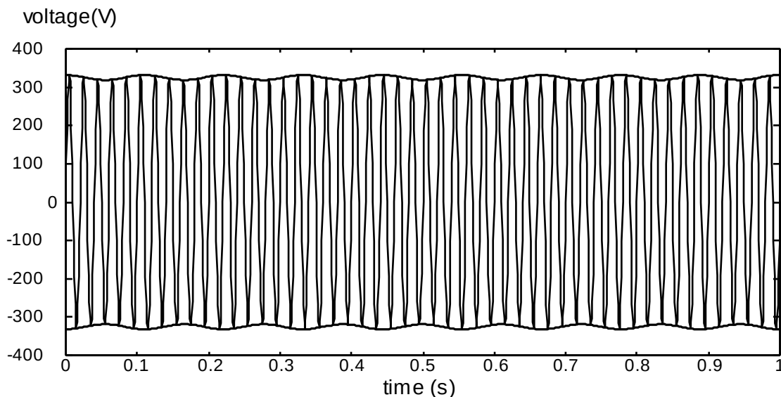
Figure 5.8: Voltage fluctuation
