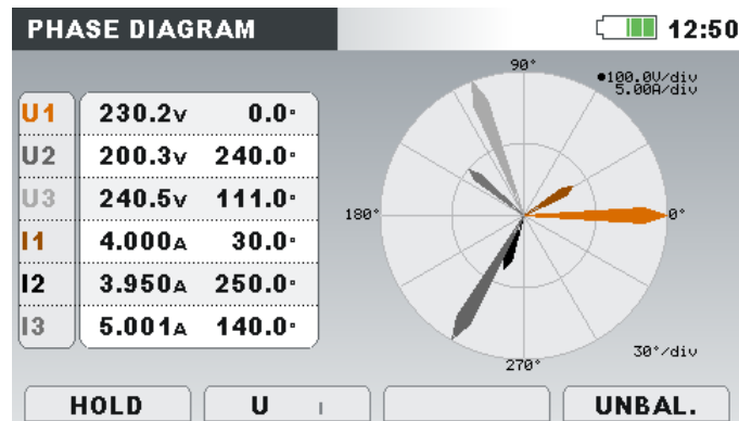
Figure 3.36: Phase diagram screen
