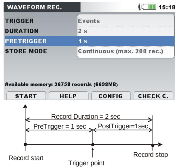
Figure 5.17: Triggering and pre-triggering description
