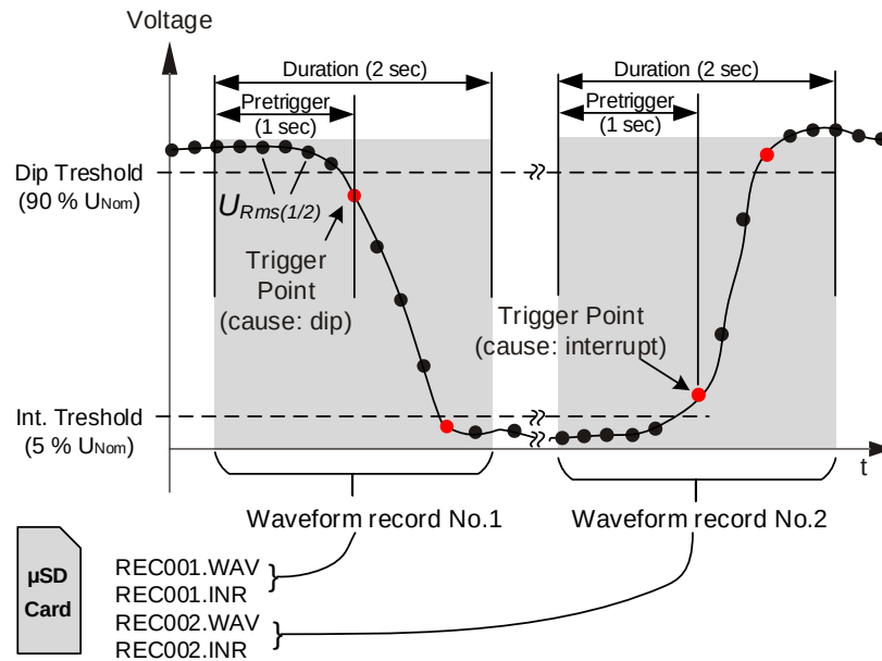
Figure 5.18: Voltage Event Triggering
