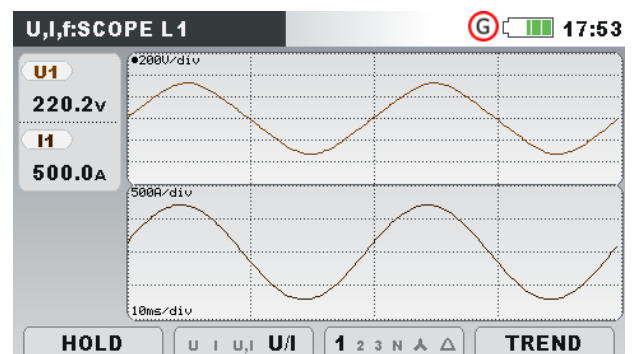
Figure 3.15: Voltage and current waveform (dual mode)
