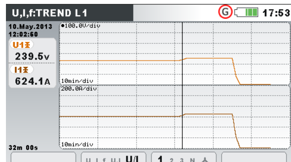
Figure 3.19: Voltage and current trend (dual mode)
