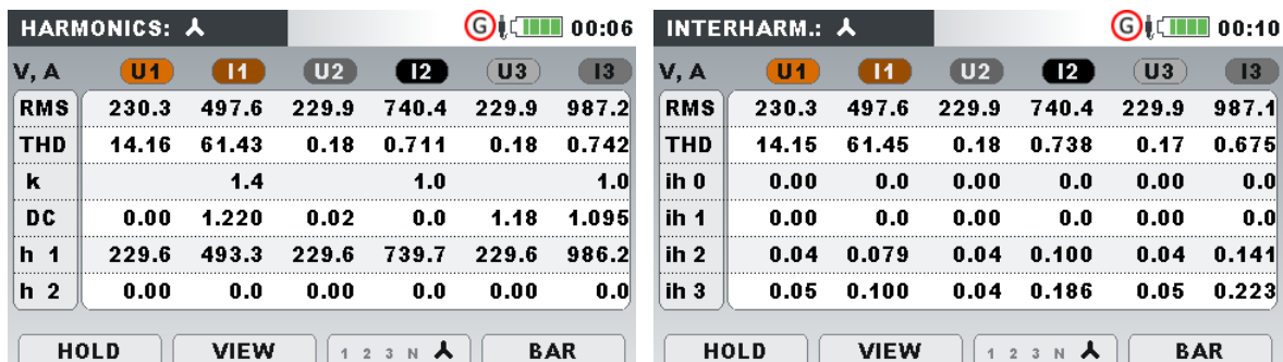
Figure 3.30: Harmonics and interharmonics (METER) screens
