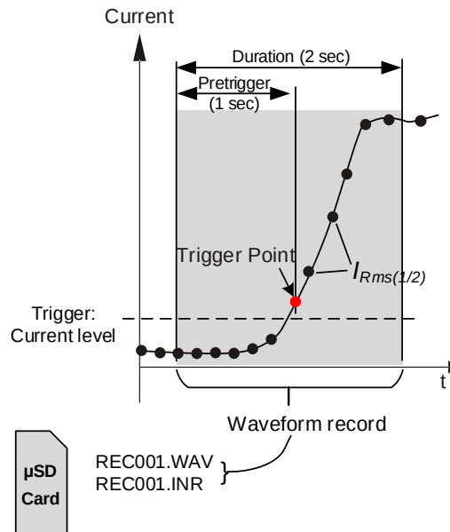
Figure 5.20: Current Level Triggering (Inrush)
