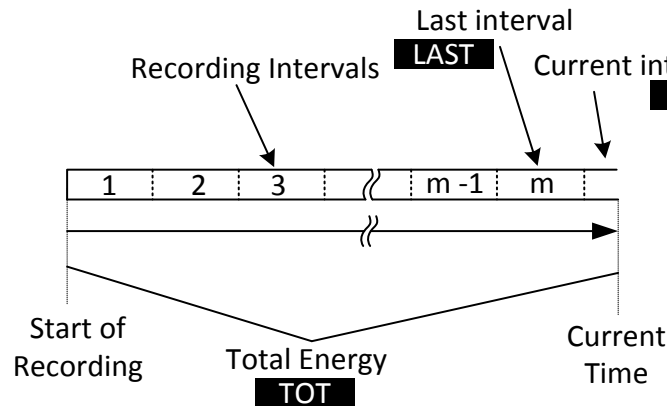
Figure 5.5: Instrument energy counters
