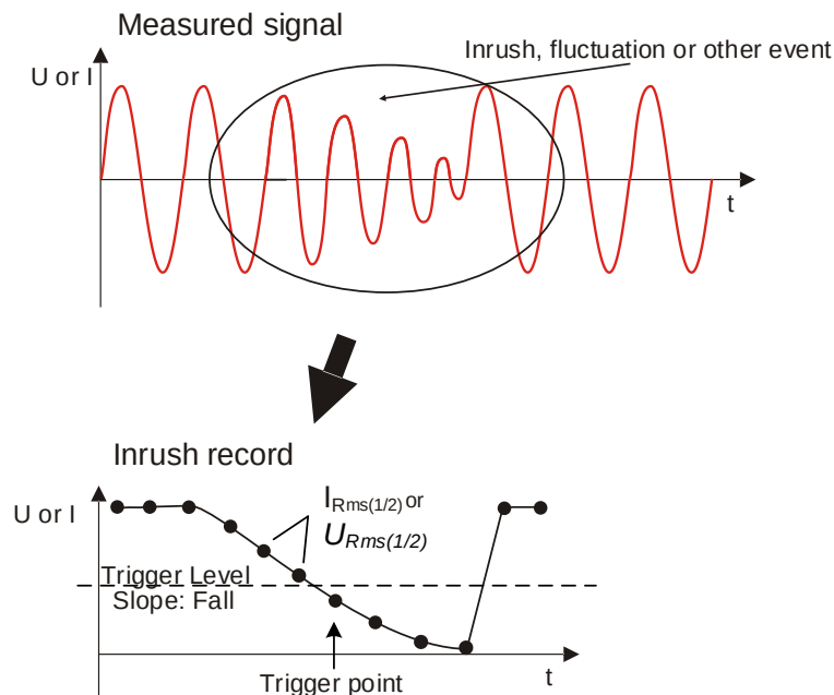
Figure 5.22: Level triggering
