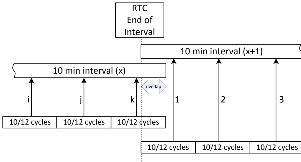
Figure 5.14: Synchronization and aggregation of 10/12 cycle intervals
