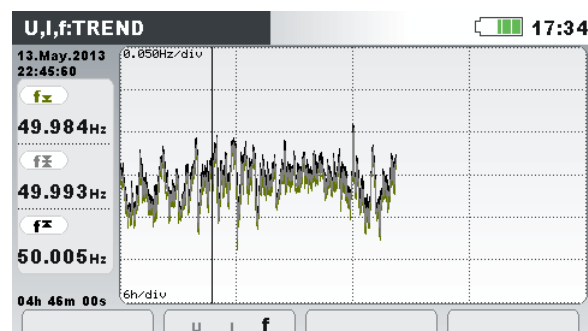
Figure 3.21: Frequency trend
