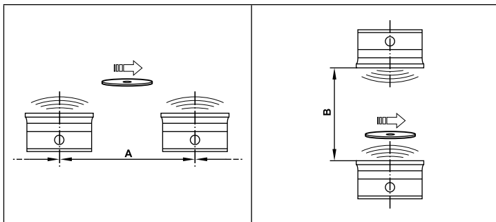
Fig. 6: Mounting distances
