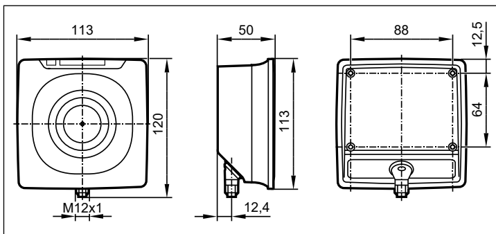
Fig. 10: Scale drawing
