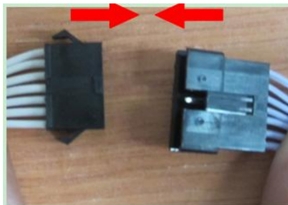
FIG-15 Connecting control panel connectors
