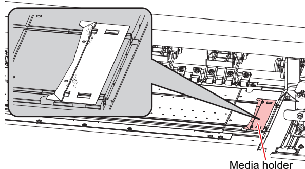
Media holder
