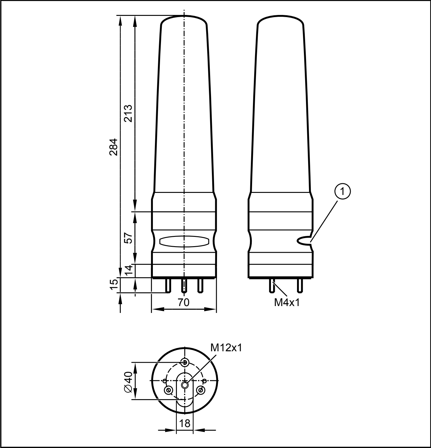
1: Buzzer Dimensions [mm]
