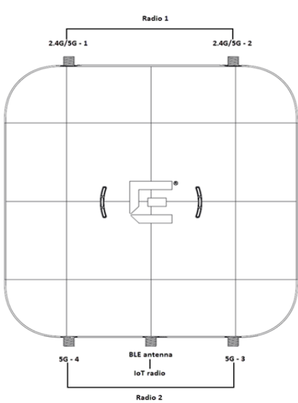
Figure 4 AP310e external antenna connectors
