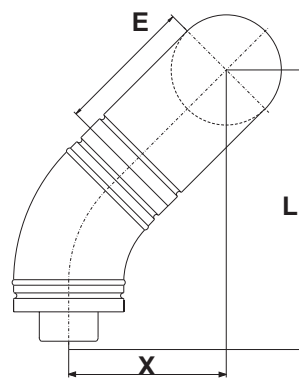
Figure 8 Single 45° elbow direct on high level balanced flue kit 90° elbow
