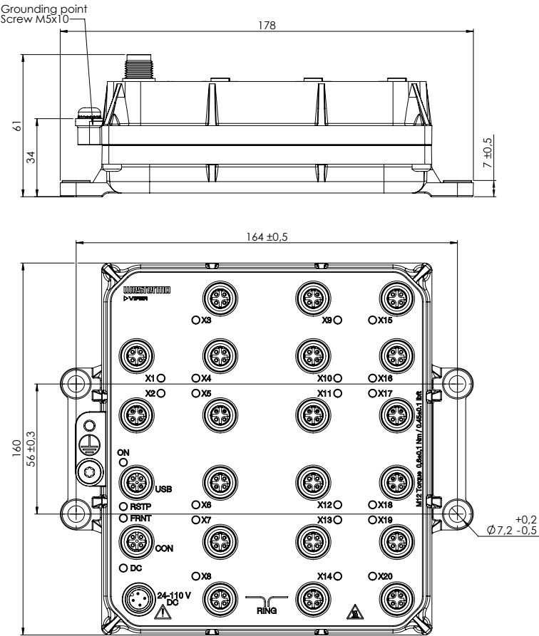
Figure 4. Dimensional drawing
