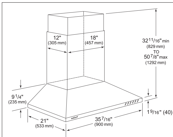
Figure 2-2 CTWH36 Dimensions
