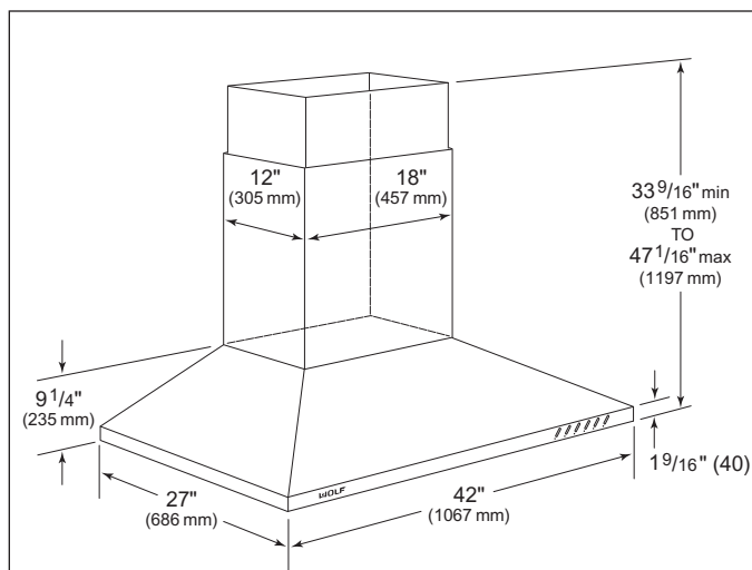
Figure 2-3 IH4227 Dimensions
