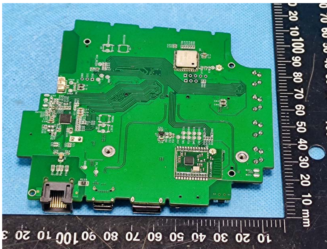
EUT- Bottom view of PCB
