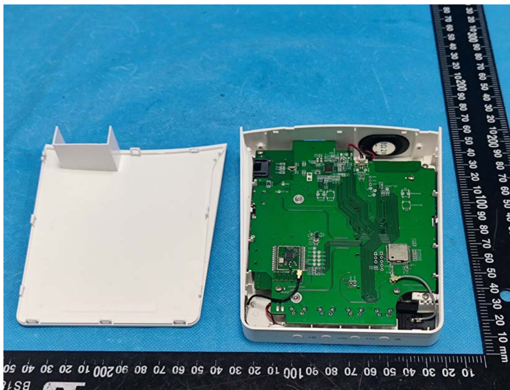
EUT-Uncover view
