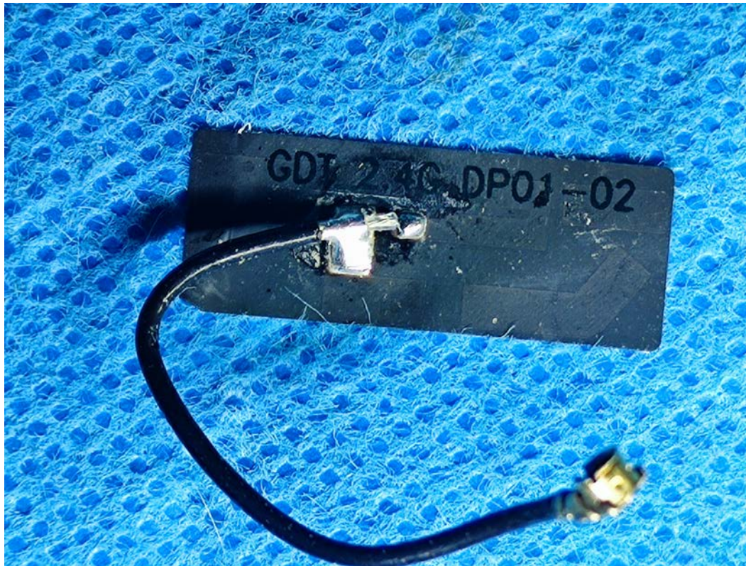
EUT- Ant view
