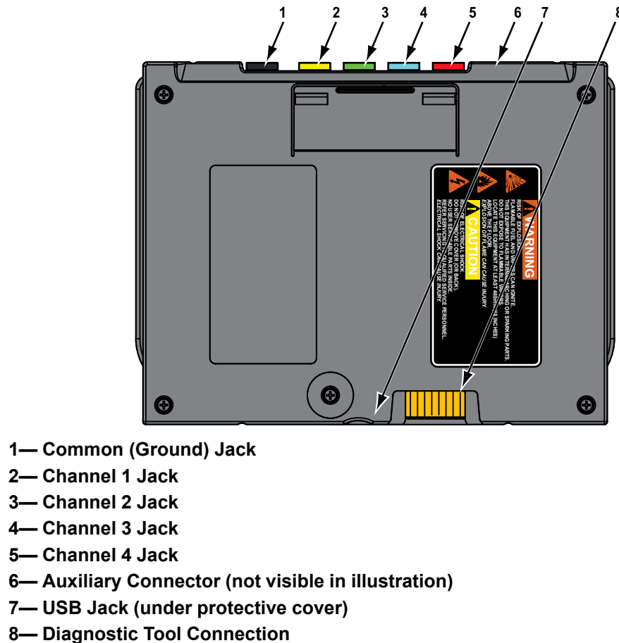
Figure 2-5 Scope Multimeter Module, removed from diagnostic tool
