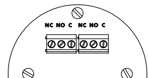
Terminal connections CSA, IECEx, ATEX enclosures
