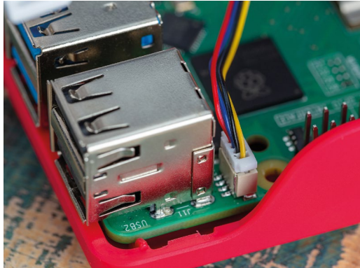
► Figure 6: Plugging in the fan connector
