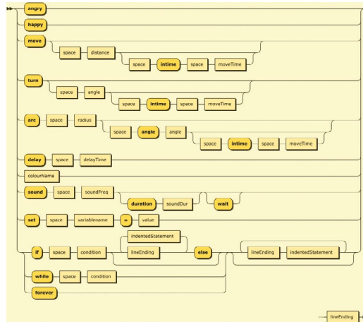
Figure 5 ♦ The diagram is created from a grammar which describes the language structure. All the details are in the language description at hullpixelbot.com
