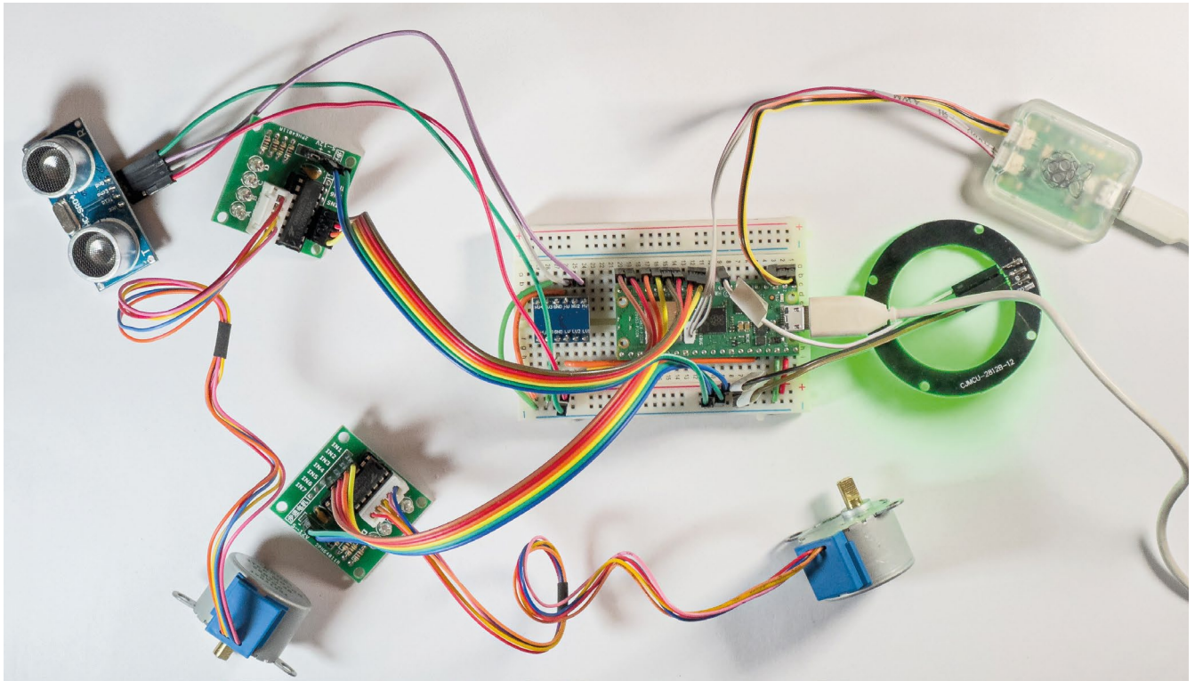
Figure 4 The C++ program that implements Python-ish is being debugged using a Pico Debug Probe. This lets us look inside the program and see what it is doing, even when it is running an interrupt handler
