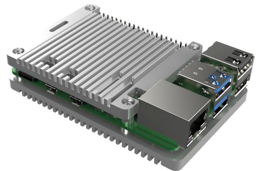
▲ The case comprises two aluminium heatsink parts that sandwich Raspberry Pi 5 between thermal pads
