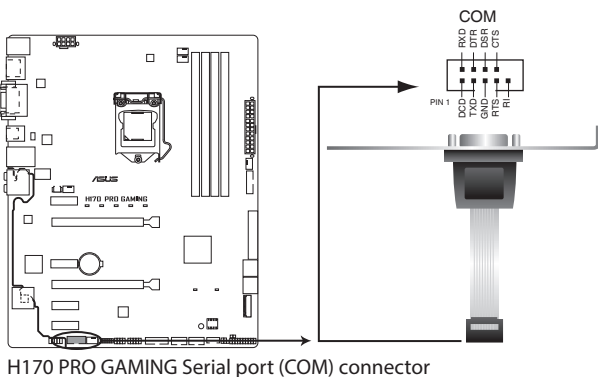
H170 PRO GAMING Serial port (COM) connector
