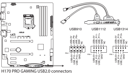
H170 PRO GAMING USB2.0 connectors
