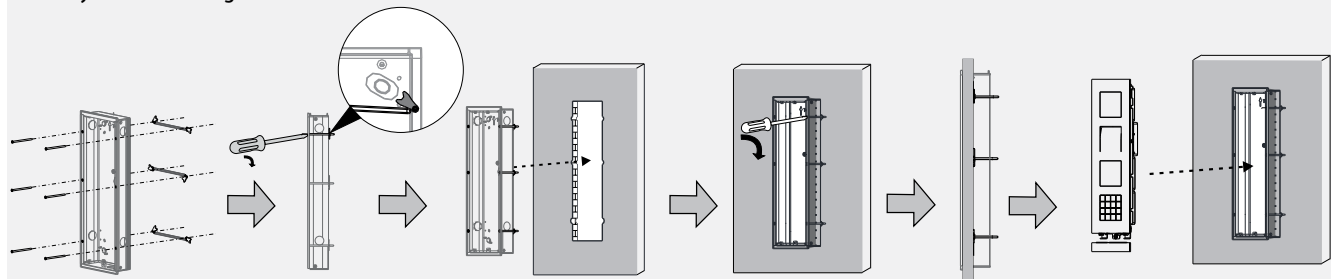
Cavity wall mounting
