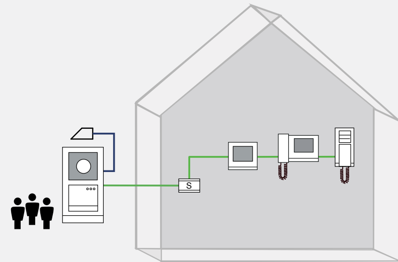
Single-family house, audio/video
