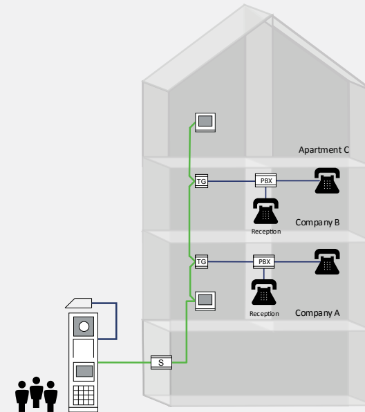
Solution for office buildings using telephones as indoor stations
