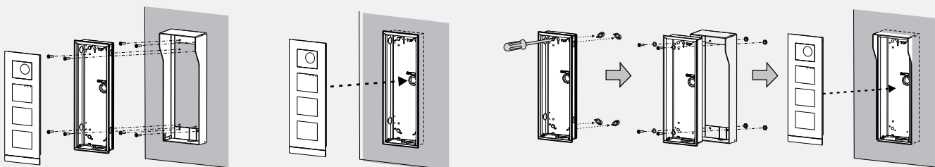
Surface-mounted with rainhood
