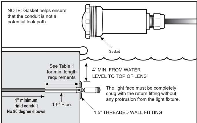
Figure 2. Standard installation with 1.5" pool wall fitting
