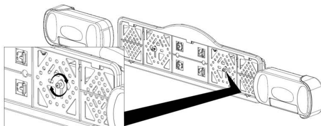
Figure 5: Mounting the license plate holder
