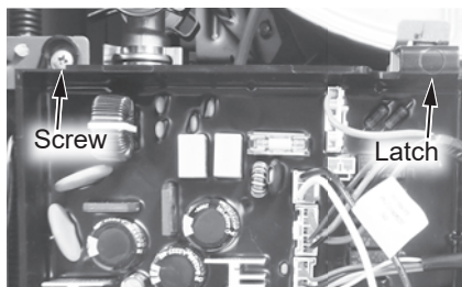
Figure 61 - Control board screw location
