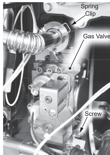
Figure 68 - Gas valve location
