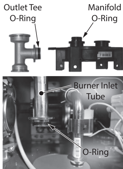
Figure 250 - Replace O-rings
