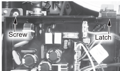
Figure 42 - Control board location
