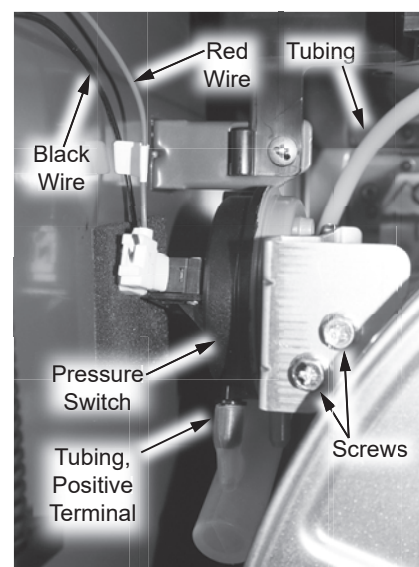
Figure 144 - Pressure switch assembly location
