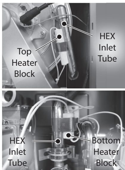
Figure 191 - Remove heater blocks from HEX inlet tube
