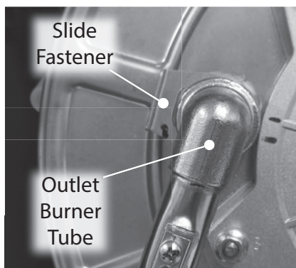
Figure 262 - Slide Fastener, Outlet Burner Tube
