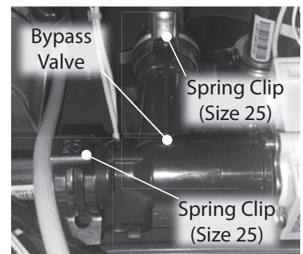
Figure 256 - Spring Clips (Size 25), Bypass Valve (B2)
