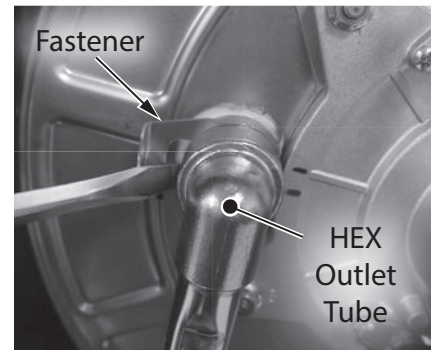
Figure 199 - Remove fastener securing HEX outlet tube
