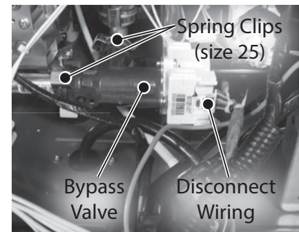
Figure 212 - Bypass valve
