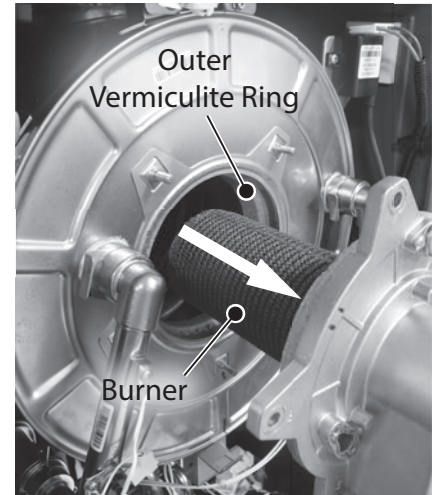
Figure 119 - Remove burner door assembly
