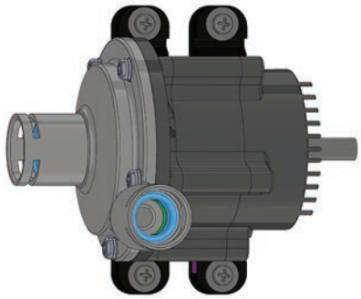
Figure 8 - Recirculation Pump
