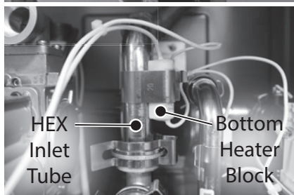
Figure 135 - Remove heater blocks from HEX inlet tube
