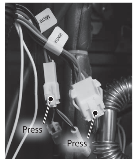
Figure 86 - Locate venturi wire harnesses
