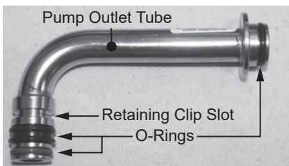
Figure 169 - Pump outlet tube O-rings
