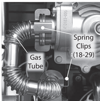
Figure 259 - Spring Clips (18-29), Gas Tube
