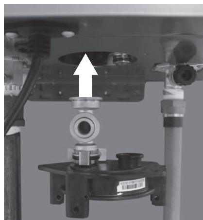
Figure 251 - Orient cartridge manifold and outlet tee
