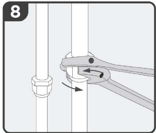
Connect Piping
