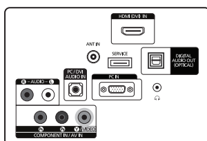
JACK PANEL DETAIL 3.6"H X 5.9"W
