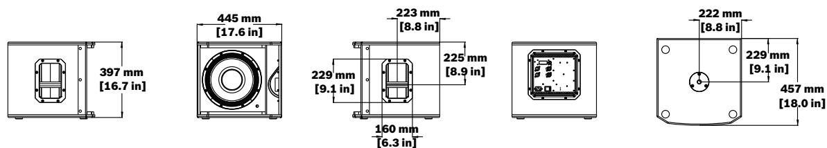
Figure 9.4: ELX200-12SP dimensions
