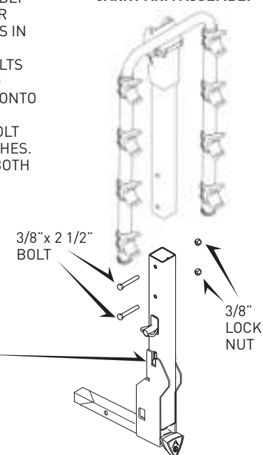
CARRY ARM ASSEMBLY
