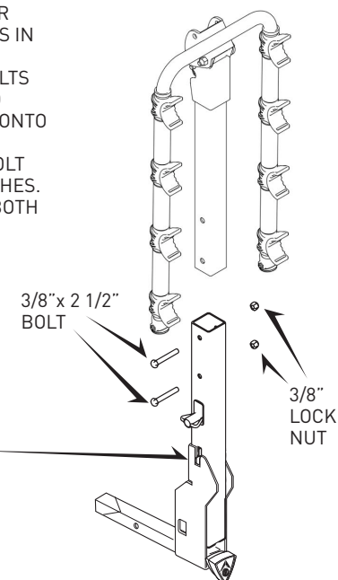
CARRY ARM ASSEMBLY
